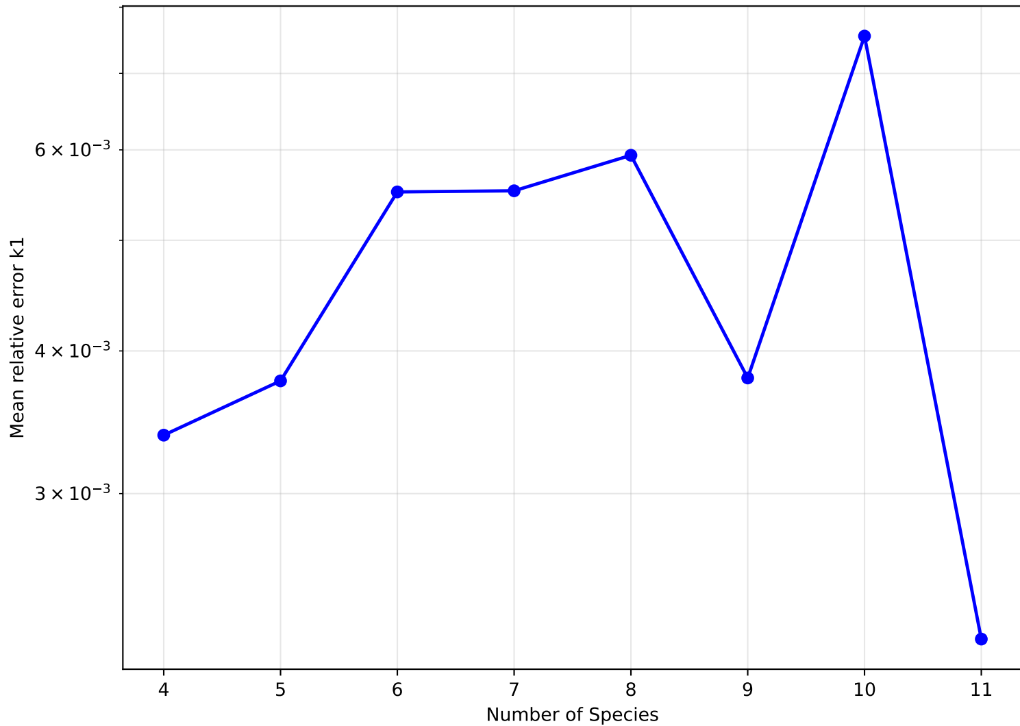
30, 30 — Mean relative error k1 vs number of species (zoomed: 4 to 11 species)
